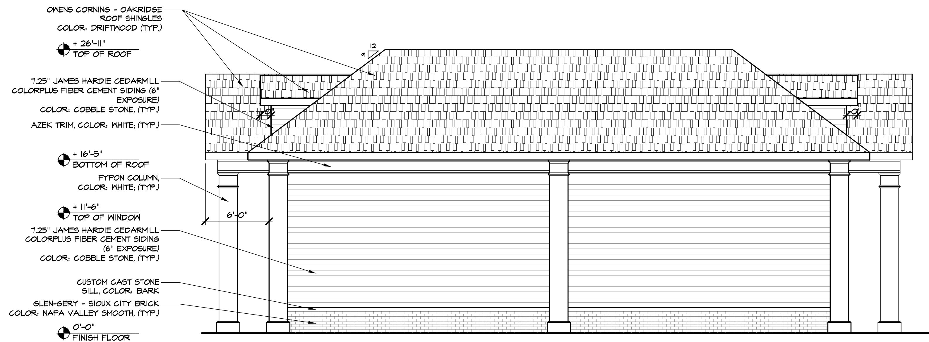
2 PROPOSED BUILDING #3 (RETAIL) - LEFT & RIGHT SIDE ELEVATION
