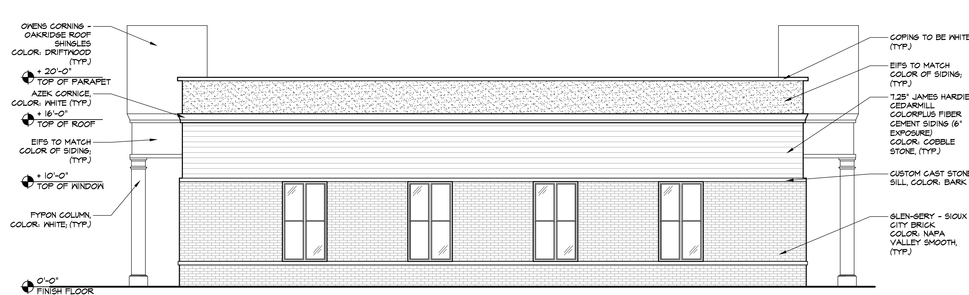
4 PROPOSED BUILDING #4 (BANK) - LEFT & RIGHT SIDE ELEVATION
